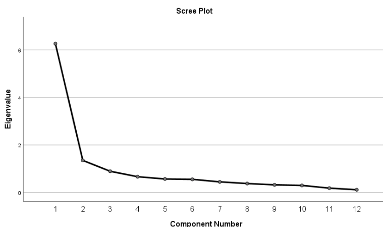
Diagram 1. Scree plot of the MANS factor structure
